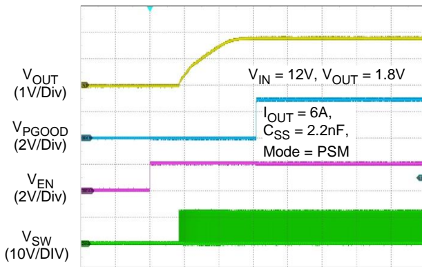
Time (1ms/Div)
