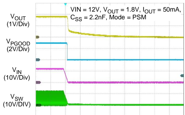
Time (5ms/Div)
