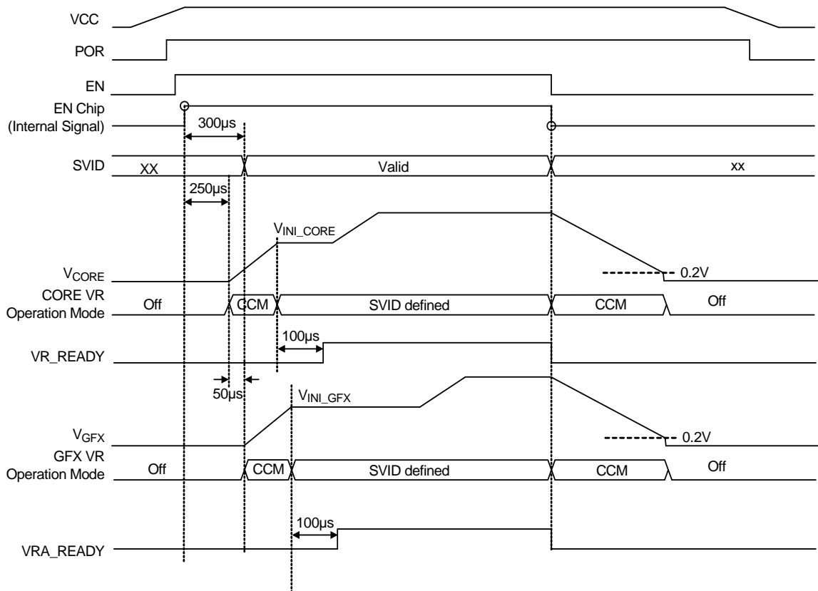
Figure 7 (b). Power sequence for RT8167B ( V_{INL\_CORE} \neq 0, V_{INL\_GFX} \neq 0V )
