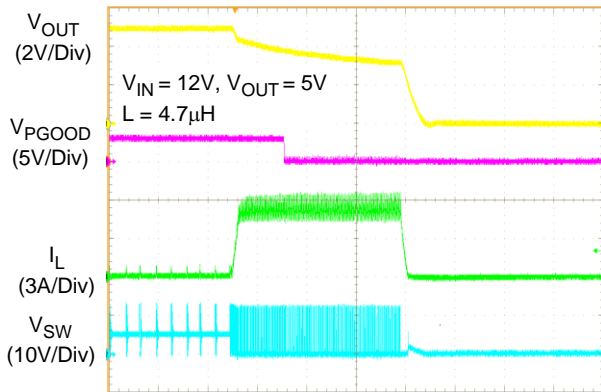
Time (50µs/Div)
