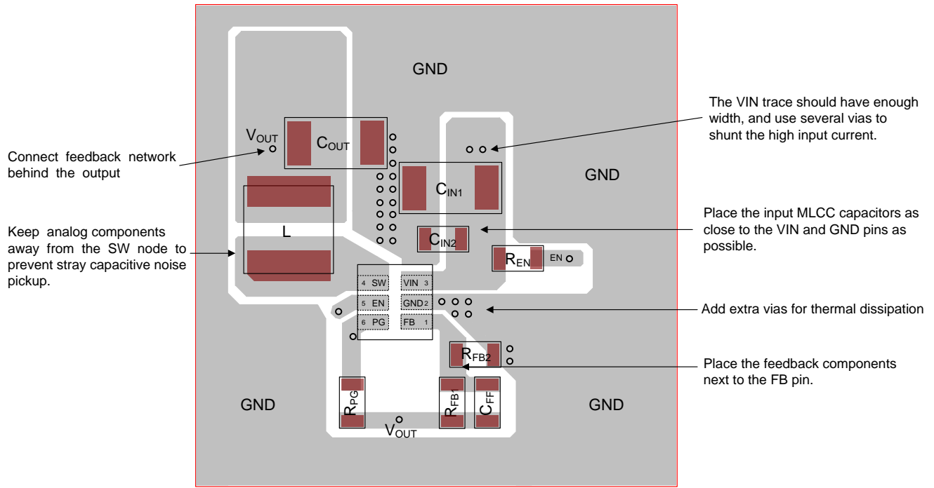
Figure 11. Layout Guide
