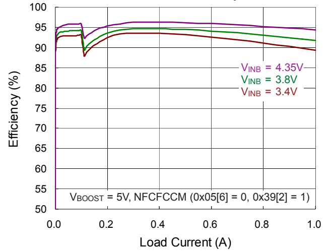
Boost Efficiency
