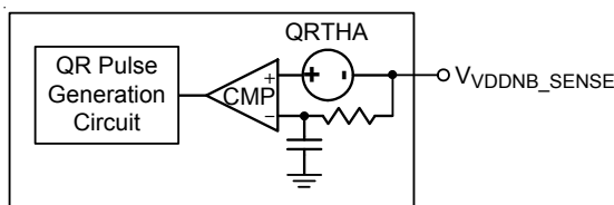
Figure 23. VDDNB Controller : Quick Response Triggering Circuit
