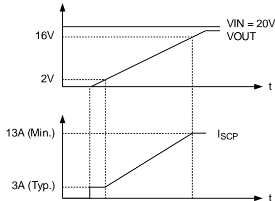
Figure 4. Short-Circuit Protection
